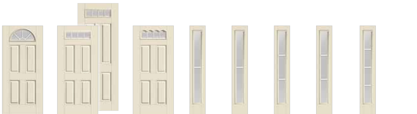
S255 * ♦ ♦ ♦ 2'8" x 6'8" 2'10" x 6'8" 3'0" x 6'8" S236 ♦ ♦ ♦ ♦ 2'6" x 6'8" 2'8" x 6'8" 2'10" x 6'8" 3'0" x 6'8" S8317 ♦ ♦ ♦ ♦ 2'6" x 8'0" 2'8" x 8'0" 2'10" x 8'0" 3'0" x 8'0" S237 * ♦ ♦ ♦ 2'8" x 6'8" 2'10" x 6'8" 3'0" x 6'8" (Scalloped Lite Frame) S1209SL * ♦ ♦ ♦ 12" x 6'8" 14" x 6'8" S1201SL * ♦ ♦ ♦ ♦ 10" x 6'8" 12" x 6'8" ‡ ‡ 14" x 6'8" ‡ ‡ S1211SL * ♦ ♦ ♦ ♦ 12" x 6'8" 14" x 6'8" S1202SL * ♦ ♦ ♦ ♦ ♦ 10" x 6'8" 12" x 6'8" ‡ ‡ 14" x 6'8" ‡ ‡ S1208SL * ♦ ♦ ♦ ♦ 6 12" x 6'8" 14" x 6'8"
